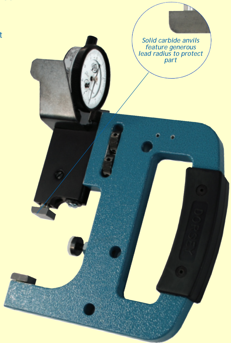
SDN-700-TR snap gage shown with optional thumb retraction
