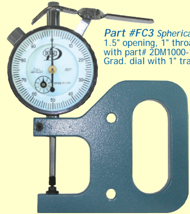
Part #FC3-NI Frame and contacts, less indicator
